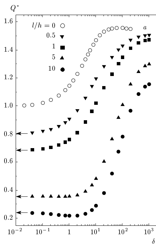
Fig. 2. a) The dimensionless mass flow rate Q^* as a function of gas rarefaction parameter \delta for various reduced channel length l/h
