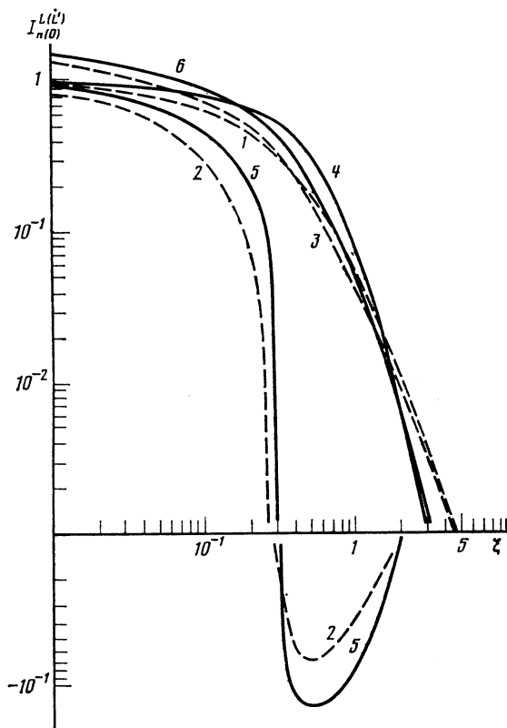
FIG. 1. Dependence of the integrals I_{nl}^{L(L')} (A1) on the Massey parameter \xi = |\Delta E| n^*/2v . Curves 1, 2, and 3—the integrals I_{n0}^s, I_{n0}^p and I_{n0}^p respectively according to (A3)–(A8); curves 4, 5, and 6—the integrals I_n^s, I_n^p and I_n^p respectively according to (A10)–(A15).
